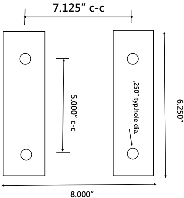
Foot print of bracket when assembled on poly board
