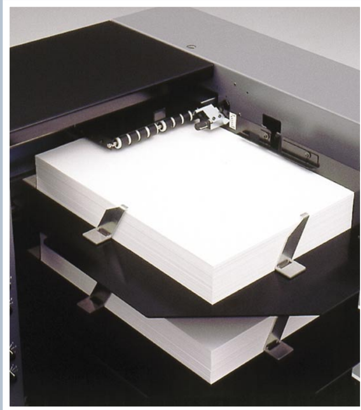
Modular Suction Feed Collator & Bookletmaker
